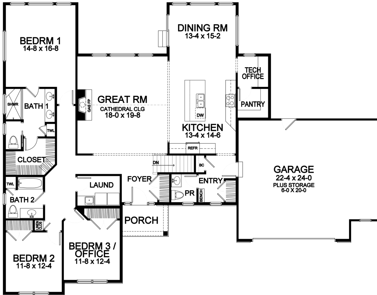
First Floor
