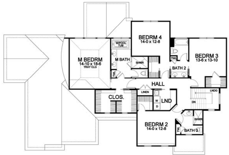
Second Floor
